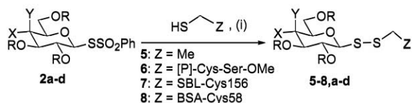
Scheme 3 Reagents and conditions: (i) for 5 DCM, Et 3 N; for 6 MeOH/DCM, Et 3 N; for 7 70 mM CHES, 5 mM MES, 2 mM CaCl 2 , pH 9.5; for 8 50 mM Tris·HCl, pH 7.7.
