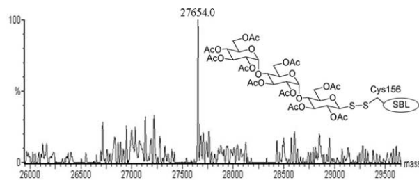
Fig. 2 ESI-MS spectrum of 7d (Found 27654, Theoretical 27649).
