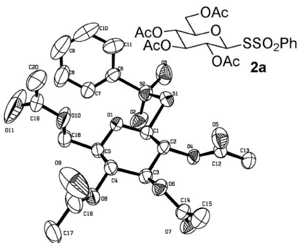
Fig. 1 Crystal structure of 2a . ¶
