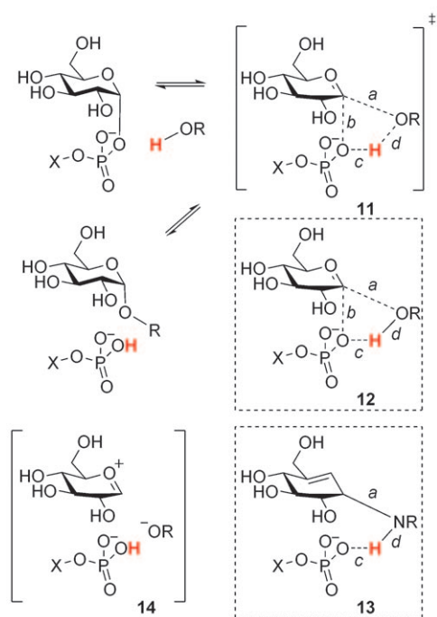
Scheme 4. An “ S_Ni -like” mechanism for retaining glucosyltransfer. The boxed ternary species 12 and 13 equate to that proposed for S_Ni and modelled by Tvaroska [4] and that seen experimentally in the OtsA complex with UDP and 4 , respectively.
