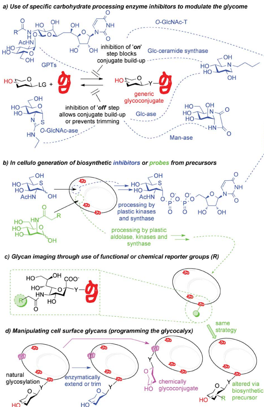
Fig. 6 Some chemical biology approaches to glycan functions.
