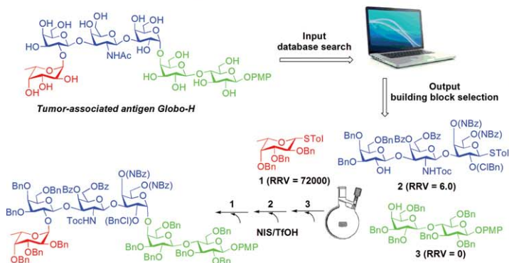
Fig. 4 Strategies for automated oligosaccharide synthesis; RRV = relative reactivity values.
