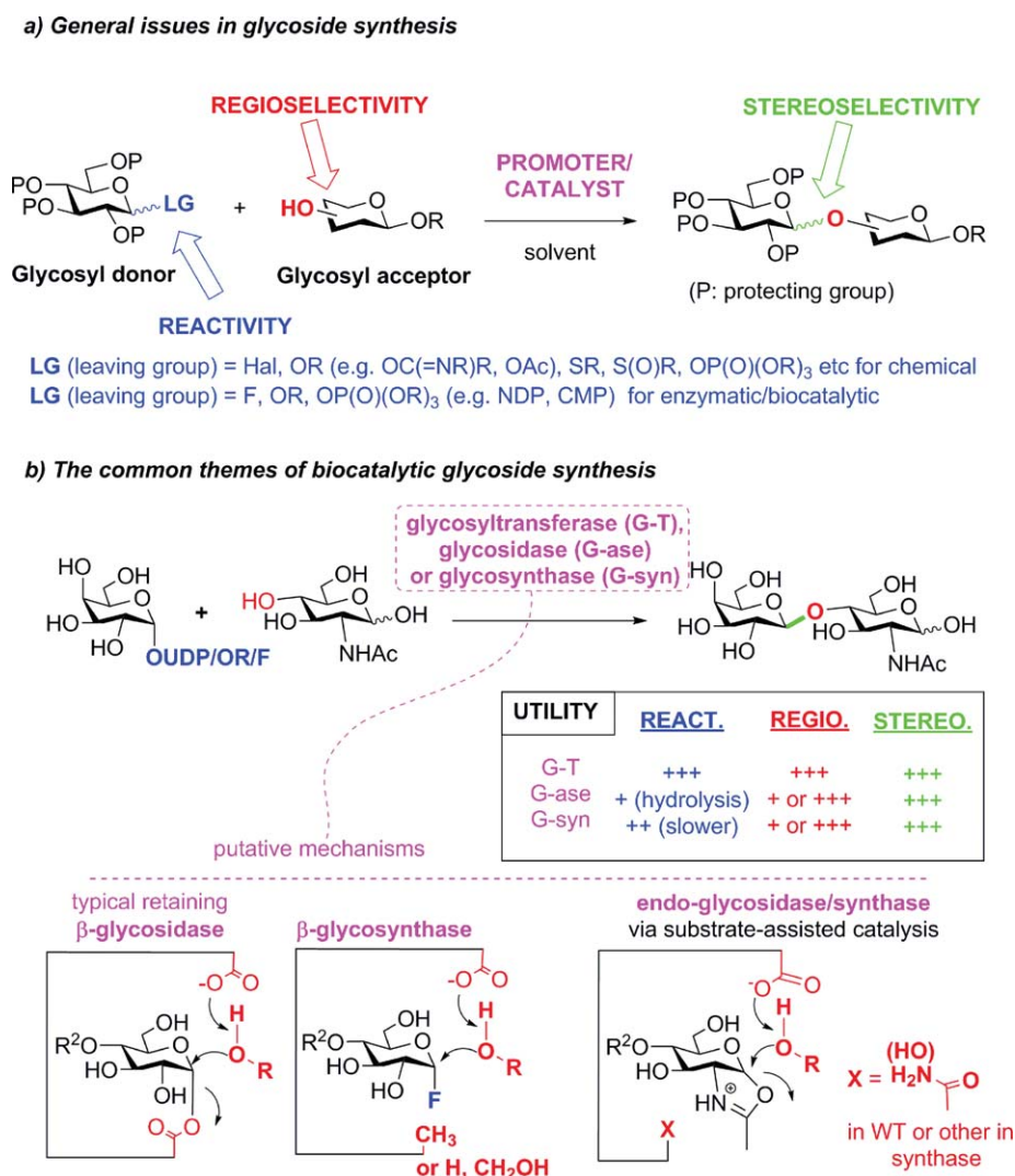
Fig. 2 Chemical and enzymatic synthesis of glycosides and oligosaccharides. (a) General issues in glycoside synthesis; and (b) the common themes of biocatalytic glycoside construction.
