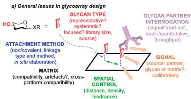
Fig. 5 General issues in glycan array design.
