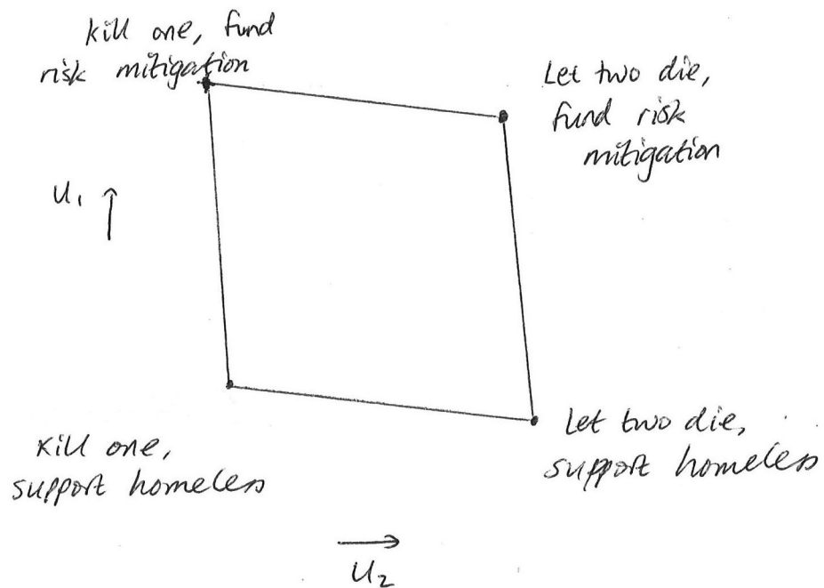
Figure 5: Two binary choices.
