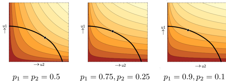
Figure 2: Nash contours and the asymmetric Nash bargaining solution (for a generic convex Pareto frontier) for various distributions (p_1, p_2) of credence between two moral theories (T_1, T_2) .
