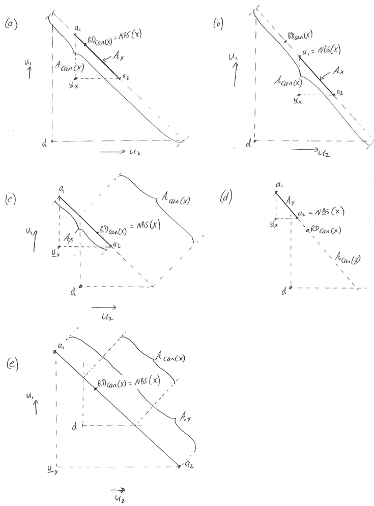
Figure 4: The Nash bargaining solution for a variety of non-canonical two-theory, two-pure-option bargaining problems. In all cases, the Nash solution NBS(X) to the problem X is the available act that is closest to RD_{Can}(X) , the Nash solution to the corresponding canonical problem Can(X) (Proposition 3).
