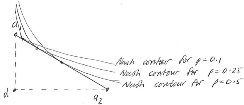
Figure 3: Illustration of Proposition 1.
