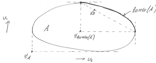
Figure 1: An arbitrary set of available options \mathcal{A} , with the Pareto frontier \text{Pareto}(\mathcal{A}) , anti-utopia point \underline{u}_{\mathcal{A}} and random dictator point RD (for the case p_1 = 0.25, p_2 = 0.75 ) labelled.
