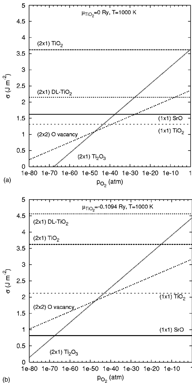
FIG. 5. Surface energies as a function of p_{\text{O}_2} at T=1000 K (a) in equilibrium with \text{TiO}_2 and (b) in equilibrium with \text{SrO} .
