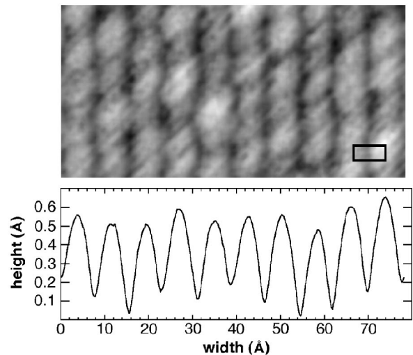
FIG. 6. STM image (2 V sample bias, 0.5 nA tunneling current) of the (2 \times 1) reconstructed surface. The two unit cell separation of the rows can be seen, but the single unit cell periodicity along the rows is not resolved. The (2 \times 1) surface unit cell is shown in the image. By averaging vertically through the image a plot of the average row heights is created as shown in the lower panel. The typical corrugation height is between 0.4 and 0.5 Å.
