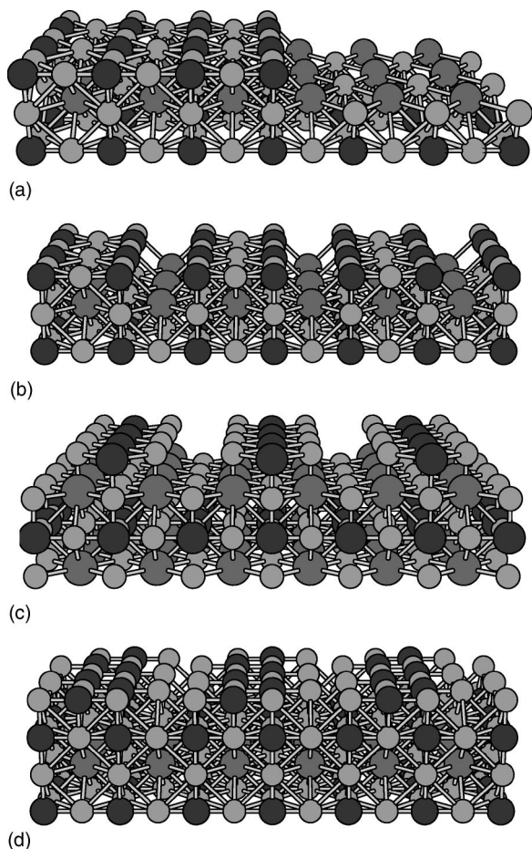
FIG. 1. (a) (1 \times 1) unreconstructed \text{TiO}_2 and SrO surfaces. (b) (2 \times 1) \text{Ti}_2\text{O}_3 reconstruction. (c) (2 \times 1) \text{TiO}_2 reconstruction. (d) (2 \times 1) DL- \text{TiO}_2 reconstruction. Ti atoms are darkest and O are lightest.
