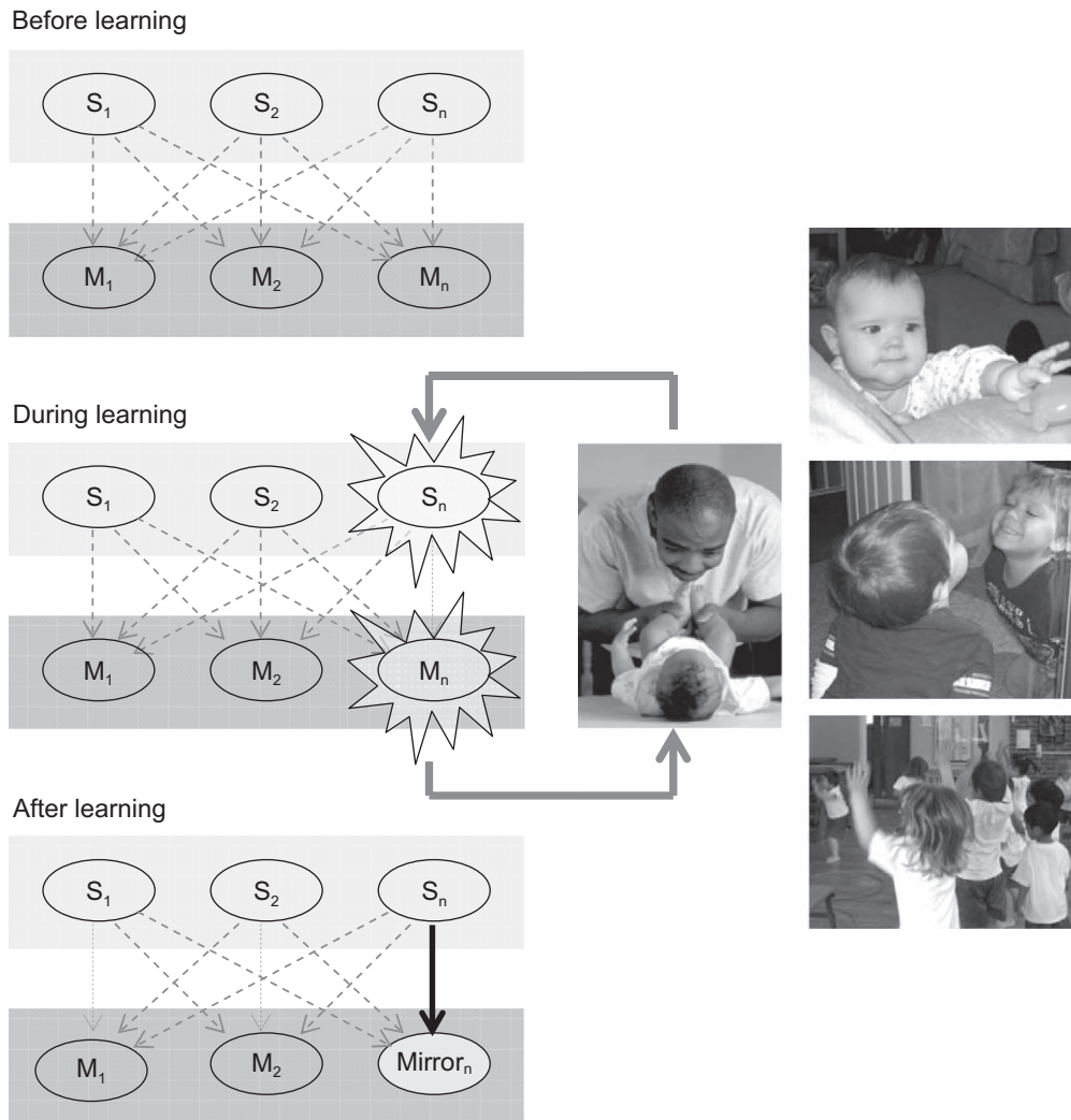
Fig. 3. The associative sequence learning account of the origin of mirror neurons (Heyes, 2010). Before learning, sensory neurons coding different types of action ( S_1 , S_2 , S_n ) are weakly and unsystematically connected to motor neurons coding different types of action ( M_1 , M_2 , M_n ). Learning occurs when there is correlated activation of sensory neurons ( S_n ) and motor neurons ( M_n ) coding similar actions (e.g., during self-observation or when an adult imitates an infant). Correlated activation of S_n and M_n increases the strength of the connection between them, so that activation of S_n is propagated to M_n . Therefore, after learning, M_n is a mirror neuron.
