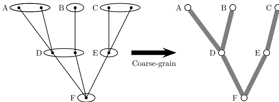
Figure 6: A coarse-graining
