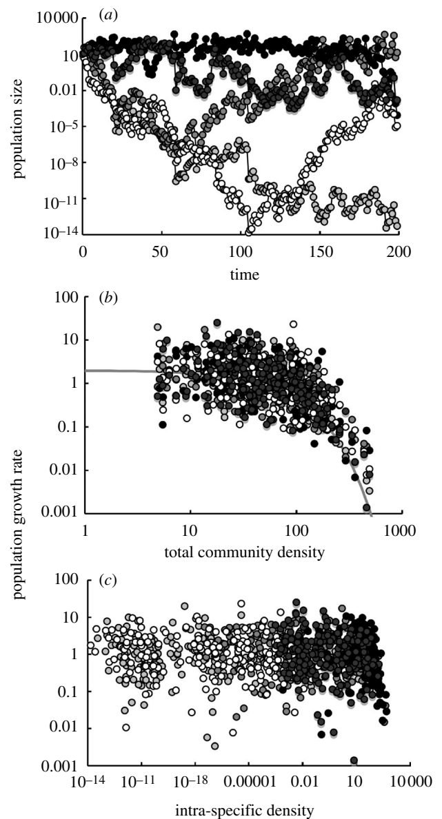
Figure 3. Example of the dynamics of a community in which density dependence acts through total community density. The five-species community was simulated using a simple model, in which the dynamics of each species was generated by a simple recurrence relationship assuming linear density dependence. Annually, densities of each species were subject to a random perturbation (lognormally distributed with geometric mean and variance of 0 and 1, respectively). (a) The dynamics of the whole community. (b) The relationship between the population growth rate of each species and the total density of the community. (c) The relationship between the population growth rate and the intraspecific density for each species.
