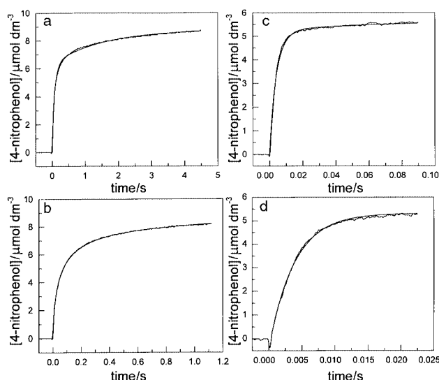
Fig. 3 Transient absorption traces recorded at 410 nm on the pulse radiolysis of either 35 or 48 ( 50 \mu\text{mol dm}^{-3} ) in an \text{N}_2\text{O} -saturated propan-2-ol-water mixture (50%, v/v) at pH 9.3 and 7.4 respectively. Panels a and b show the biphasic reductive elimination of 4-nitrophenol on two different timescales when a dose per pulse of 15.5 Gy equivalent to [(\text{CH}_3)_2\text{C}^{\cdot}\text{OH}] = 10.4 \mu\text{mol dm}^{-3} was used. Panels c and d show the reductive elimination of 4-nitrophenol from the semiquinone radical of 48 on two different timescales when [(\text{CH}_3)_2\text{C}^{\cdot}\text{OH}] = 5.4 \mu\text{mol dm}^{-3} . Each of the kinetic traces is overlapped by a simulated trace which best fits the experimental data.
