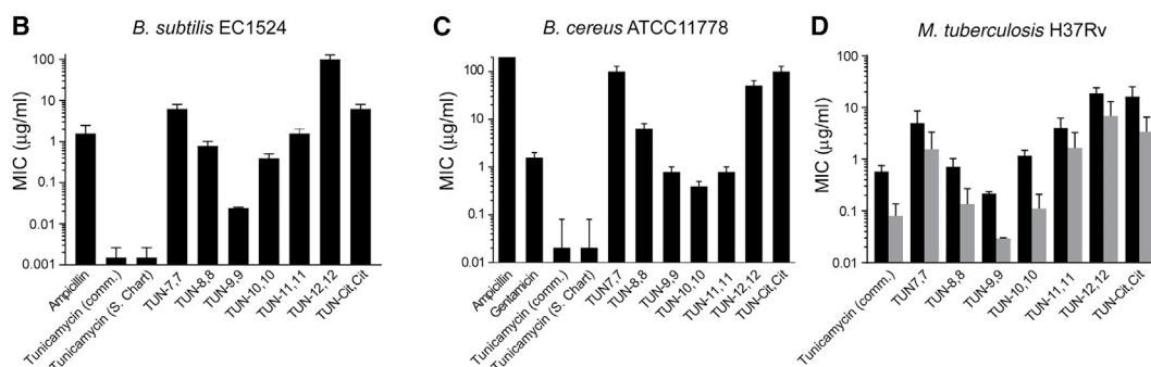
Figure 5. Semi-synthetic Synthesis and Antibacterial Effects of TUN-X,X Analogues
