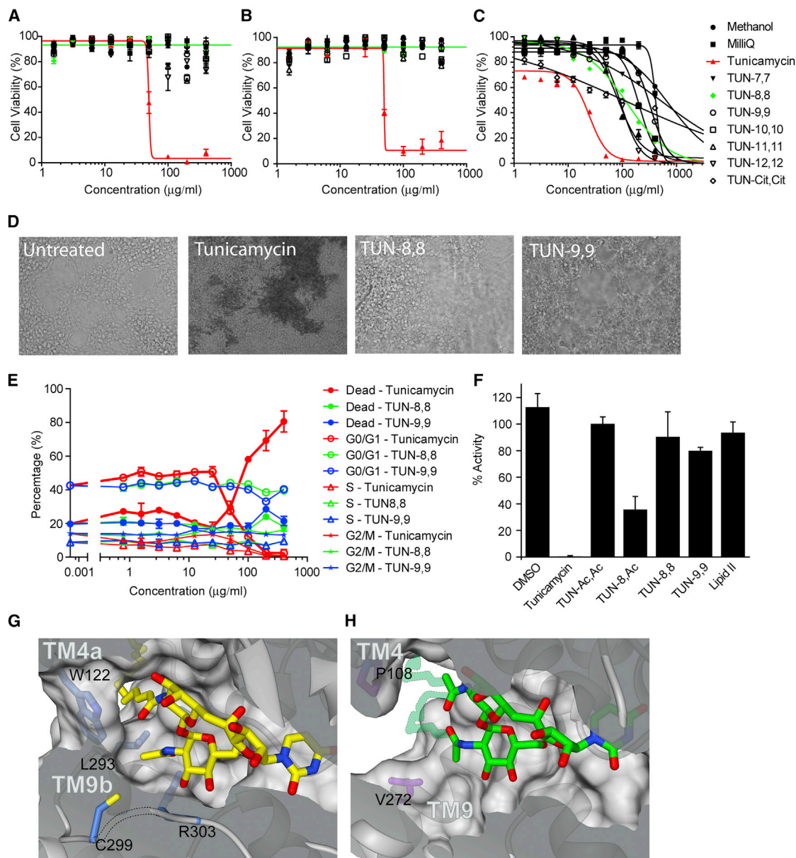
Figure 6. TUN-X,X Analogues are Not Toxic to Cultured Human Cells
