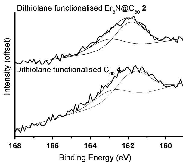
Fig. 9 S2p core level peak in XPS spectra of self-assembled monolayers of dithiolane functionalised \text{Er}_3\text{N}@C_{80} ( 2 ) and dithiolane functionalised C_{60} ( 4 ) on Au(111). The peak intensity is offset for clarity. Gaussian peak fits are included.
