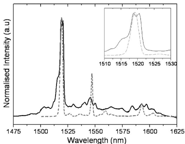
Fig. 7 Photoluminescence spectra of 2 (solid) and Er 3 N@C 80 (dashed) in CS 2 solutions at 5 K under 532 nm excitation. The inset shows the most intense emission line at ~1520 nm in greater detail, highlighting the splitting of 2 .
