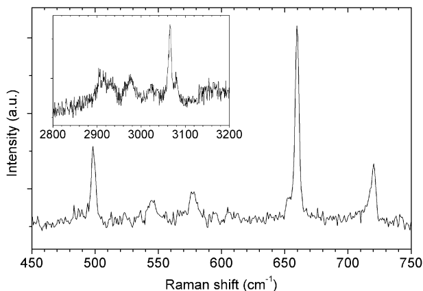
Fig. 6 Raman spectrum of 2 under 532 nm laser excitation, confirming the functionalisation. Raman shifts in the ranges typical for CS–SC (main plot), and C–H (inset) bond associated vibrations are shown.
