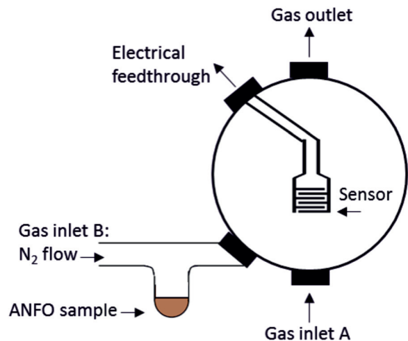
Fig. 1 Schematic of the sensing chamber showing the position of the sensor, electrical feedthrough for resistance measurements, gas outlet, gas inlet A, and gas inlet B with the t-shaped attachment for solid and liquid samples; an ANFO sample in this example.
