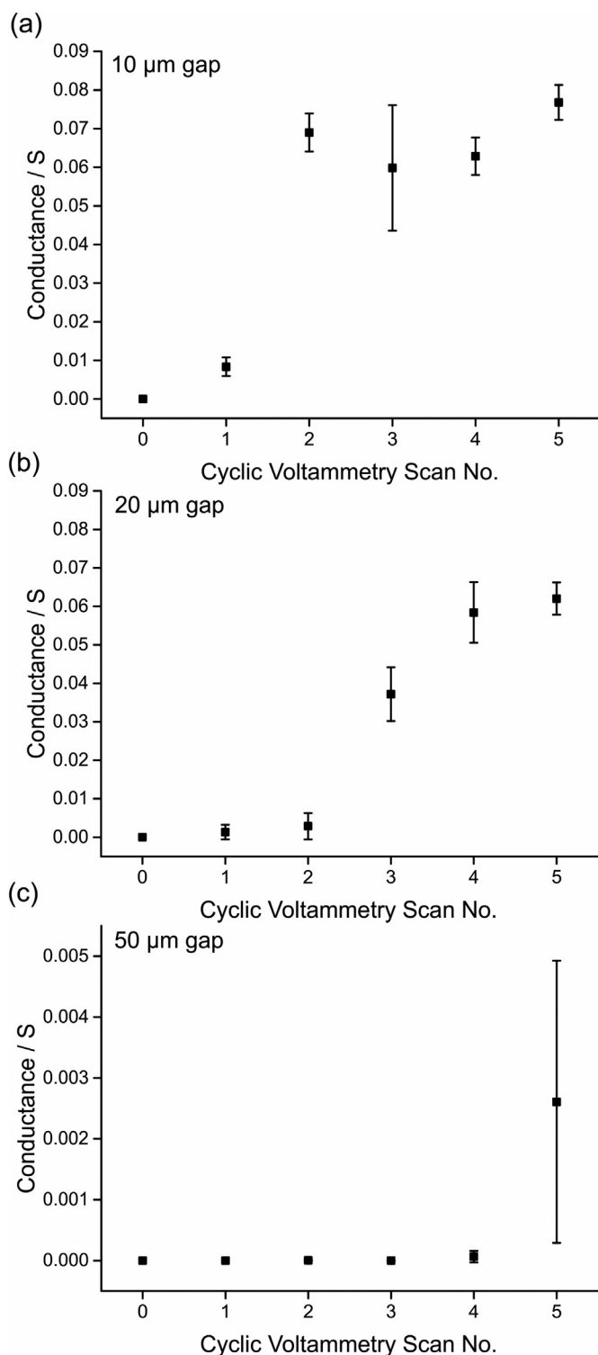
Fig. 3. Conductance vs CV scans for IDEs with gap widths of a) 10 \mu\text{m} , b) 20 \mu\text{m} and c) 50 \mu\text{m} . Error bars are obtained from the standard deviation of the conductance values of three electrode measurements for each CV scan. Thus the data in this figure is the result of 45 separate experiments, each using a fresh IDE.
